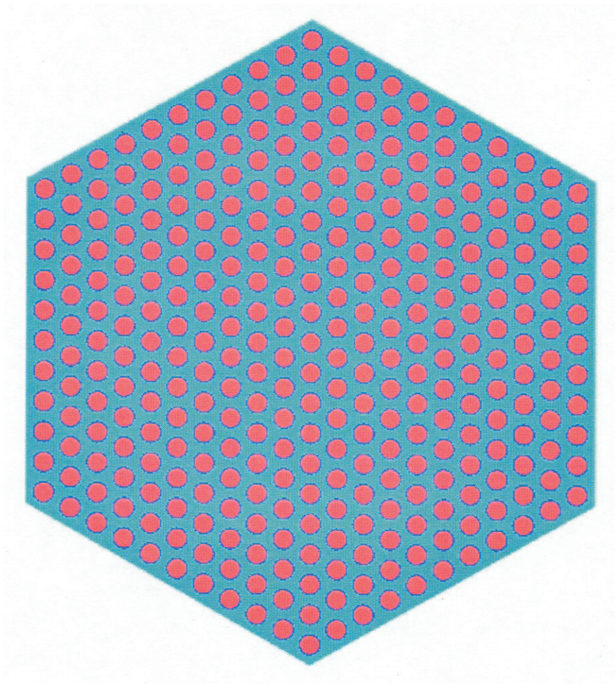
Figure 2.2.4. MOX or UO 2 hexagonal assembly.
