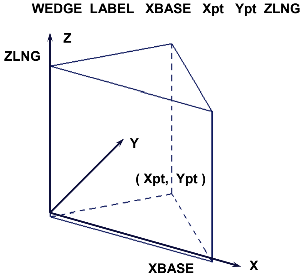
Figure 8.1.B.16. Example of wedge construction.
