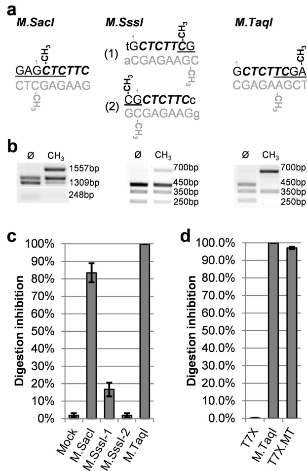
Figure 3. EarI sensitivity to methylation. (a) Methylases studied with their respective binding sites (underlined) and targeted residues (–CH 3 ) on forward (black) and reverse (gray) strands. The EarI recognition site is indicated in bold/italic and position number 1 of the 5' GCTCTTC3' site is indicated in gray numbering. (b) Agarose gel showing methylation-dependent inhibition of EarI activity. Left panel: M.SacI was expressed in E. coli T7Express (T7X) and the expression plasmid carrying the site shown in a (pET28-M.SacI) was subjected to EarI digestion. Sensitivity is expressed by accumulation of the 1557 bp band (1309 bp + 248 bp). Middle and Right panels: distinct 1055 bp PCR products carrying each site shown in a (M.SssI-1 or M.TaqI, respectively) were methylated in vitro and subjected to EarI digestion. Sensitivity is expressed by accumulation of the 700 bp band (450 bp + 250 bp). Images are representative of duplicated experiments. (c) Gel bands of each replicate described in b were quantified and expressed as percentage: 1 - [\text{digested}/(\text{digested} + \text{linearized})] in each tube. Mock is average of non-methylated DNAs (n = 6) and bars are standard error. Non methylated sites in the same molecule showed the digestion was >97% completed in each tube. (d) Methylation efficiency of 5,291 bp (M.Test) vector in vivo by T7X.MT (which carries the TaqI methyltransferase in the genome, see Supplementary Fig. 3) compared to control (same vector in T7X) and in vitro data (M.TaqI; similar to c but new replicates). T7X.MT carrying the plasmids were selected on plates supplemented with 0.3mM IPTG and grown overnight at 37°C in liquid media + 0.2 mM IPTG for 14–18 h before DNA extraction. Bars are standard error of four biological replicates and graph is a representative image of a duplicated experiment.
