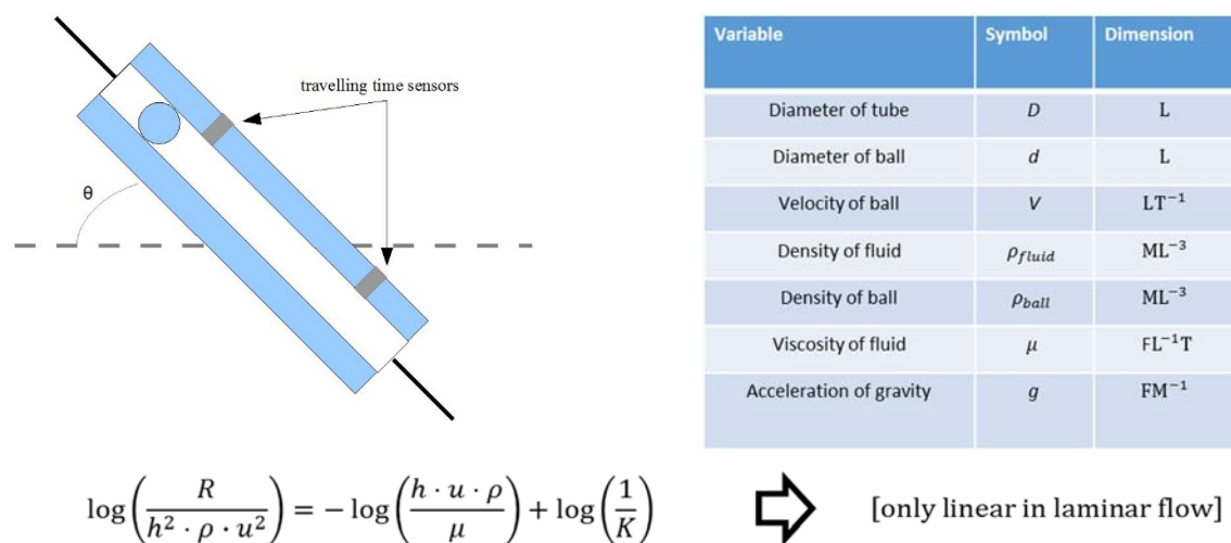
Figure 6. Miniature rolling-ball viscometer description. | Image courtesy of Prof. Uday Pal, Boston University
