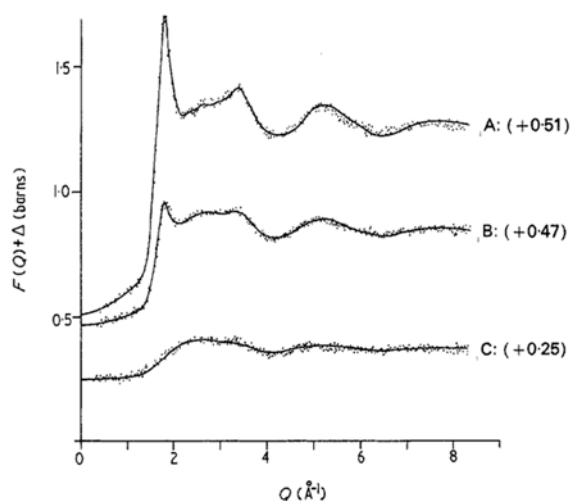
Figure 11. Total structure factor, F(Q) , data for liquid \text{Na}^{35}\text{Cl} (curve A), NaCl (Curve B), and \text{Na}^{37}\text{Cl} (Curve C) at 875 °C. The points are the experimental data and the curves are derived from the partial structure factors | Reproduced from F. G. Edwards, J. E. Enderby, R. A. Howe, and D. A. Page. "The structure of molten sodium chloride." J. Phys. C: Solid State Phys. 8(21), 3483–3490, 1975, http://iopscience.iop.org/article/10.1088/0022-3719/8/21/018/pdf
