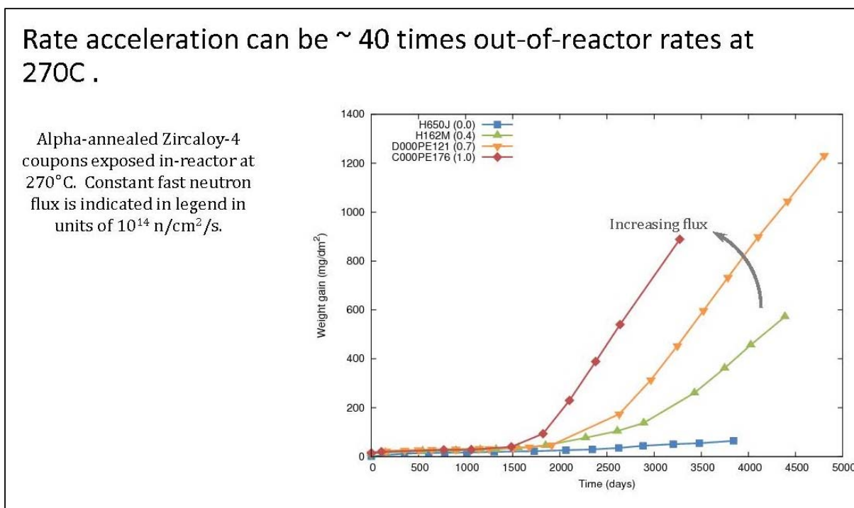
Figure 26. Irradiation enhancement of corrosion rates. | B. F. Kammenzind, J. A. Gruber, R. Bajaj, and J. D. Smee. "Neutron irradiation effects on the corrosion of Zircaloy-4 in a PWR environment." Paper B-T-3965, 18th International Symposium on Zirconium in the Nuclear Industry, Hilton Head, South Carolina, May 15–19, 2016. Used by permission.
