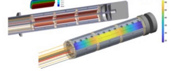
Dose Rate (Mrad/hr)
