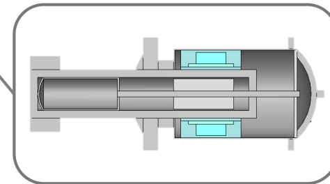
Stirling Engine
