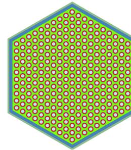
Fuel Assembly
