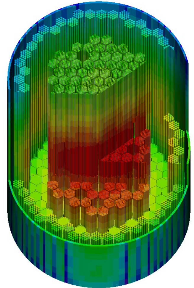
Neutron flux (cladding, coolant, reflector rod, removed)
