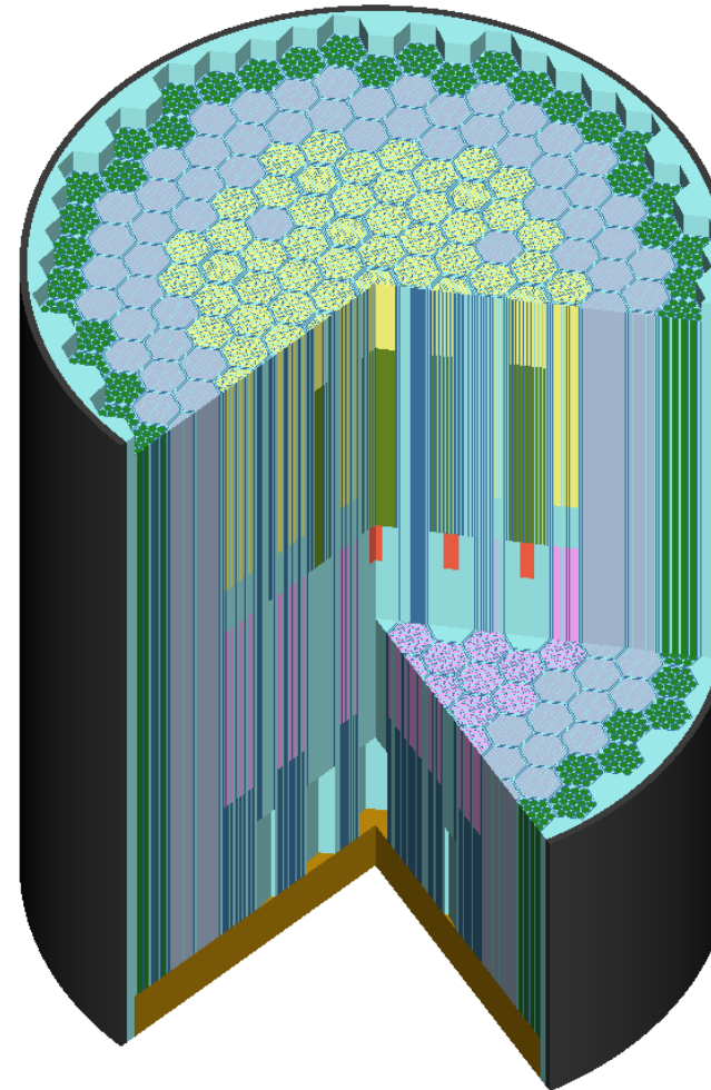
3D SCALE model
