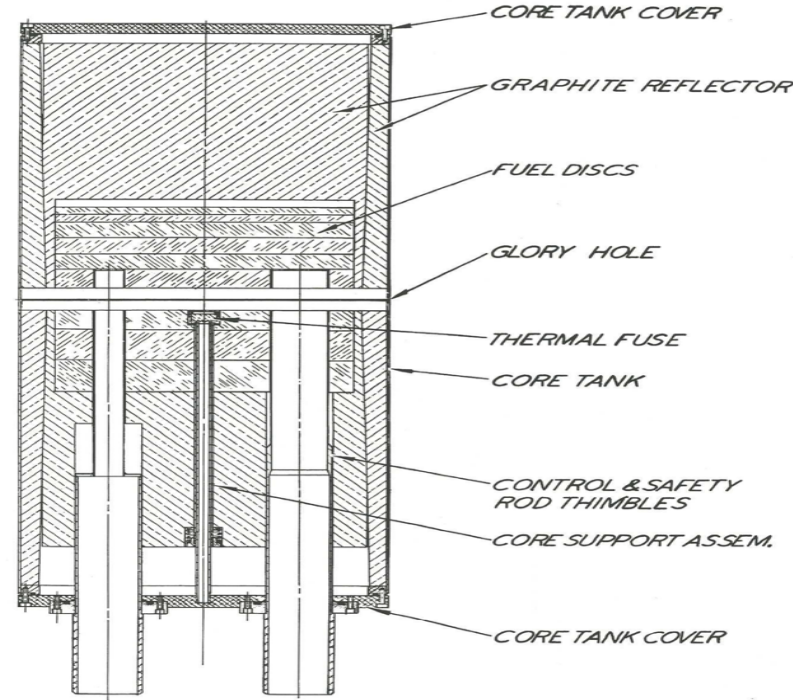
Original AGN-201M reactor
