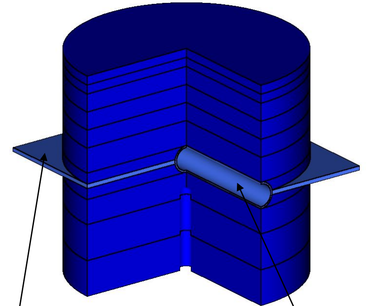
Baffle plate and glory hole configuration
