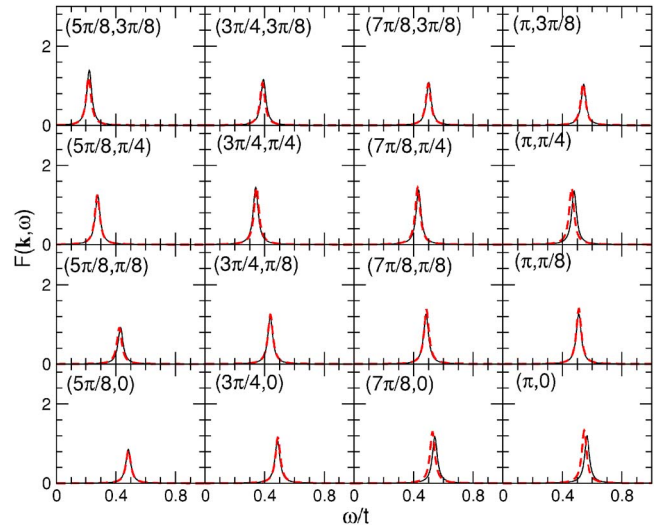
FIG. 3. (Color online) The same as in Fig. 2 but for N = 240 ( n \approx 0.94 ) (Ref. 21). The momentum-independent renormalization factor z_B is 0.18.
