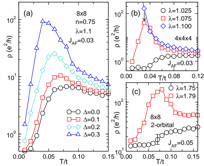
Figure 6. Monte Carlo results reproduced from [9], where more details can be found, emphasizing the role of quenched disorder and also including three-dimensional and two-orbital effects. (a) \rho vs. T in the presence of quenched disorder \Delta . Up to ten different disorder realizations were used in calculations with quenched disorder. Only small changes between configurations were observed. Monte Carlo steps and starting configurations are as in Fig. 4. (b) \rho vs. T using a 4 \times 4 \times 4 lattice, parametrized with \lambda , at J_{AF}=0.03 . (c) Two orbitals \rho vs. T results using an 8 \times 8 lattice for J_{AF}=0.05 . In (b) and (c), 4000 thermalization and 4000 measurement Monte Carlo steps were used, n=0.75 , and the clean limit \Delta=0 was studied.
