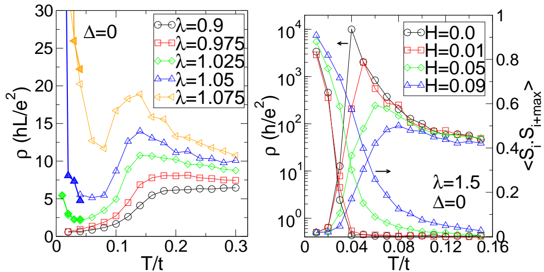
Figure 3. Left : Influence of the electron-phonon coupling \lambda in the clean limit \Delta=0 on the resistivity curve using a 4 \times 4 \times 4 lattice at density n=0.3 . The model used was the one-orbital Hamiltonian with J_{AF}=0 . Reproduced from [7], where more details can be found. Right : Influence of magnetic fields on the resistivity curve and on the spin-spin correlation at the maximum allowed distance ( 4\sqrt{2} ) on an 8 \times 8 lattice in the clean limit \Delta=0 , at n=0.1 . These results are reproduced from [7].
