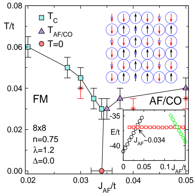
Figure 4. Clean limit Monte Carlo phase diagram using 8 \times 8 and 12 \times 12 lattices, at n=0.75 and \lambda=1.2 , reproduced from Ref. [9], where more details can be found. The AF/CO state is schematically shown, with the radius of the circles proportional to the electronic density, and arrows representing the t_{2g} spins. Charge is uniform in the competing FM state. At each temperature, 10^5 thermalization and 5 \times 10^4 measurement Monte Carlo steps were carried out for the 8 \times 8 clusters (and \sim 7500 and 5000 , respectively, for the 12 \times 12 cluster points indicated by red stars). Inset: energy vs. J_{AF} at very low T \sim 0 , with the FM (CO/AF) phase denoted by black circles (red squares). Green diamonds indicate a G-type AF regime.
