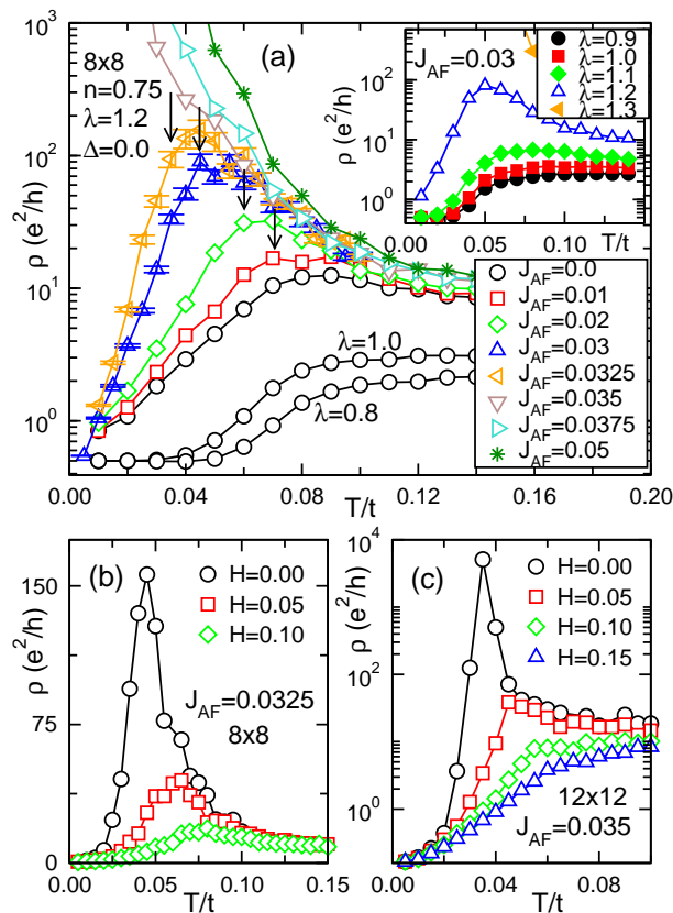
Figure 5. Resistivity \rho vs T curves for various parameters: (a) Fixing \lambda=1.2 and varying J_{AF} . Arrows indicate T_C 's. Results at \lambda=0.8 and \lambda=1.0 , with J_{AF}=0.0 , are also shown. Inset : results fixing J_{AF}=0.03 and varying \lambda . (b) Effect of magnetic fields (indicated, in t units) on \rho using J_{AF}=0.0325 , on an 8 \times 8 lattice. (c) Same as (b) but for J_{AF}=0.035 , on a 12 \times 12 lattice. These results are reproduced from [9], where more details can be found.
