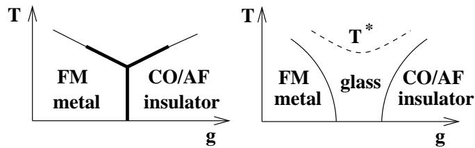
Figure 1. Schematic representation of the ideas described in [1, 2, 3] to understand the CMR effect. In the left panel, the proposed phase diagram of manganites in the clean limit is presented. This involves a first-order transition from a FM metal to a CO/AF insulator. In the right panel, the modified phase diagram is shown after the inclusion of disorder. The glassy region above the Curie temperature of the FM metallic phase is the regime where the CMR effect is proposed to occur.
