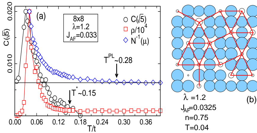
Figure 7. (a) Monte Carlo averaged C(\sqrt{5}) (charge-charge correlation at distance \sqrt{5} ) vs. T , showing a qualitative similarity with the resistivity \rho (shown). This agreement occurs below the T^* indicated. At higher T , \rho is flat and C(\sqrt{5}) nearly vanishes. Also shown is the inverse of the density of states N(\omega = \mu) , to indicate the formation of a pseudogap at T^{pl} . (b) Typical Monte Carlo snapshot with the radius of the circles proportional to the local charge density. Also shown are the hole-hole distances \sqrt{5} and 2 of relevance (see text and [9]).
