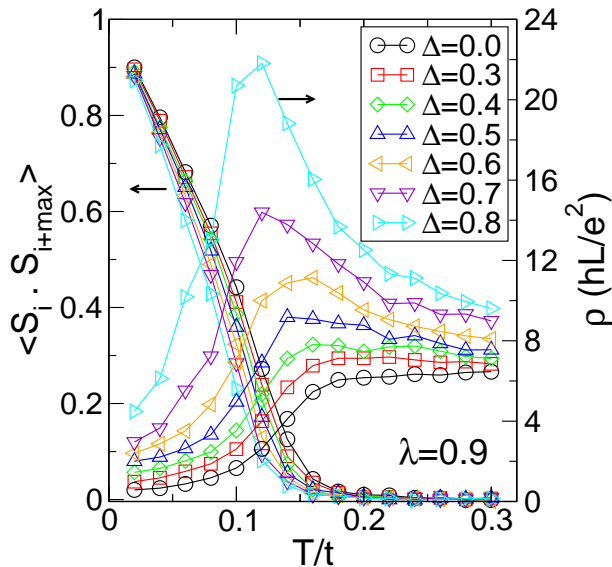
Figure 2. Monte Carlo results obtained using a 4 \times 4 \times 4 lattice. Shown are the resistivity and spin-spin correlations, the latter at the maximum allowed distance ( 2\sqrt{3} ) vs. temperature ( T ), working with the one-orbital model at electron-phonon coupling \lambda=0.9 and electronic density n=0.3 , and for the disorder strengths \Delta indicated. The results shown are mainly for one configuration of quenched disorder, but as many as 10 configurations were used in particular cases of temperatures and \Delta 's, and no substantial deviations were observed between disorder configurations. These are results reproduced from [7].
