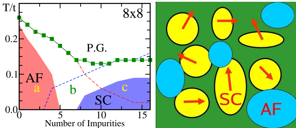
Figure 9. Left : Phase diagram of the phenomenological model used in Ref. [5], after introducing quenched disorder (for details see [5]). The disorder was introduced via plaquette impurities, mimicking Sr-doping in single-layers. \text{Sr}^{2+} replaces \text{La}^{3+} , above the center of a Cu-plaquette in the Cu-oxide square lattice, donating a hole. Then, as hole carriers are added, a hole-attractive plaquette-centered potential is also incorporated. Near the center of this potential, n should be sufficiently reduced from 1 that, phenomenologically, tendencies to SC should be expected. By this procedure, the horizontal axis labeled “Number of impurities” is concomitant with hole doping. The Monte Carlo phase diagram is shown, indicating the presence of a region b where there is no dominant order, as opposed to the AF in a and SC in c . The “P.G.” line denotes the region with a pseudogap in the density-of-states. Right : Schematic representation of the “glassy” state that separates the SC and AF regions, according to the study in [5]. The arrows indicate the phase of the SC order parameter in the many patches. Reproduced from [5].
