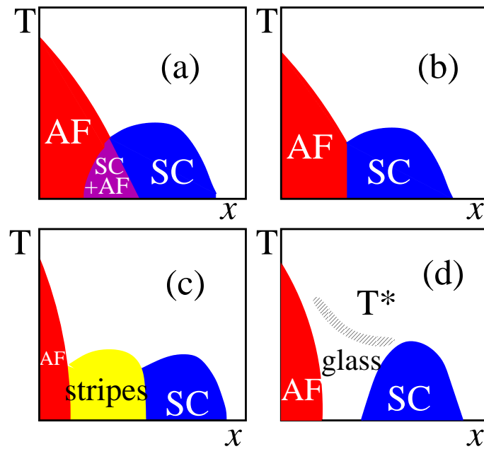
Figure 10. Schematic representation of the phase diagrams that the model studied in [5] present in the clean (a,b,c) and dirty (d) limits. In the clean limit, regions with local coexistence of AF and SC (panel a), or a first-order transition separating AF from SC (panel b) with the first-order character of the transition possibly continuing in the AF-disordered and SC-disordered transitions, or an intermediate striped regime (panel c), are possible. None reproduces the phase diagram of cuprates with an intermediate glassy state. This is achieved only by adding quenched disorder (see panel d). In this regime, a T^* temperature is found below which a pseudogap exists in the density-of-states. This phase diagram has similarities with those proposed before for manganites [1, 2], and certainly it is in excellent agreement with the experimental phase diagram of LSCO. For more details, see [5].
