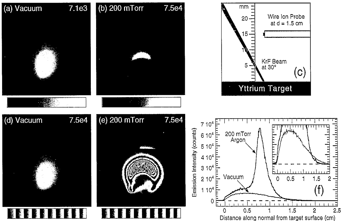
Fig. 2. Gated ICCD photographs of the total visible optical plasma emission during \Delta t = 1.00\text{--}1.05 \mu\text{s} following 0.8 \text{ J/cm}^2 KrF-laser irradiation of yttrium metal into (a) 1 \times 10^{-6} Torr and (b) 200 mTorr argon. The peak of the grayscale palette is normalized to 7100 and 75000 counts, respectively. (c) Schematic indicating the side-on view of the yttrium target, mm scale, and wire-ion probe position at d = 1.5 cm. (d), (e). The same photographs are replotted with a 10-grayscale palette and equal normalization to 75000 counts for direct comparison. A line-profile of the emission intensity from the irradiated spot along the target normal (f) shows the correct relative scaling between the vacuum and background images. The inset in (f) more clearly shows the same data replotted on a 0–8000 count scale to illustrate the small, but resolvable emission in 200 mTorr argon out to and beyond 1.5 cm.
