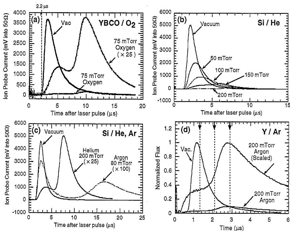
Fig. 1. Ion probe current waveforms measured along the normal to various targets at the indicated delays following 248 nm KrF-laser ablation in vacuum and background gas: (a) Y_1Ba_2Cu_3O_{7-x} into 75 mTorr oxygen, 1.5 \text{ J/cm}^2 , 2 \text{ mm} \times 2 \text{ mm} spot, d = 5 cm (b) Silicon into helium, 2.8 \text{ J/cm}^2 , d = 5 cm, actual voltages (c) Silicon into helium (200 mTorr) and argon (80 mTorr), 2.8 \text{ J/cm}^2 , 3.2 \times 2.0 \text{ mm} spot, d = 5 cm, voltages scaled by 25 and 100, resp. to illustrate the relative timing between vacuum and ‘fast’ component arrival times (d) Yttrium into 200 mTorr argon, 0.8 \text{ J/cm}^2 , 2.0 cm line focus, d = 1.5 cm. The bimodal 200 mTorr waveform is plotted in correct magnitude relative to the vacuum pulse and replotted scaled by a factor of 10. The peak of the vacuum pulse corresponds to a current flux of 25 \text{ A/cm}^2 . Imaging and optical absorption spectroscopy were performed at the three times indicated in 200 mTorr argon.
