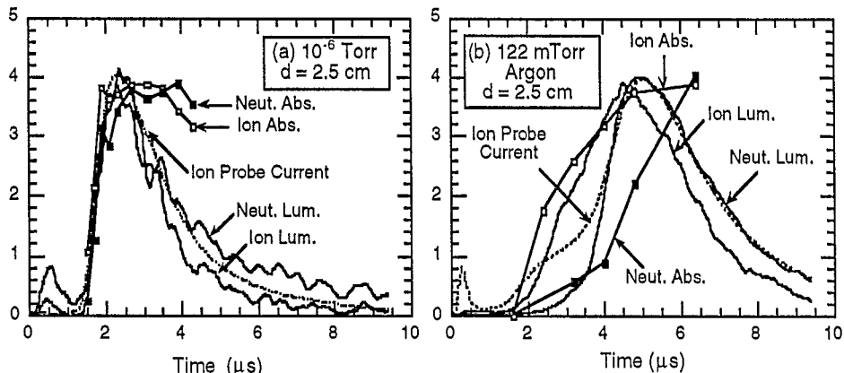
Fig. 4. Normalized ion probe current (IP), luminescence (Lum.) intensities of Y^* (410.2 nm) and Y^{++} (363.3 nm), and optical absorbances (Abs.) of Y (362.1 nm) and Y^+ (363.3 nm) at d = 2.5 cm following 0.8 \text{ J/cm}^2 KrF-laser irradiation of yttrium in (a) vacuum ( 1 \times 10^{-6} Torr) and (b) 122 mTorr argon. Scaling factors: (a) Lum: Y^* ( \times 3 ), Y^{++} ( \times 1 ), abs: Y ( \times 70 ), Y^+ ( \times 94 ), IP (mV/81), (b) lum: Y^* ( \times 23 ), Y^{++} ( \times 12.5 ), Abs: Y ( \times 100 ), Y^+ ( \times 70 ), IP (mV/81).
