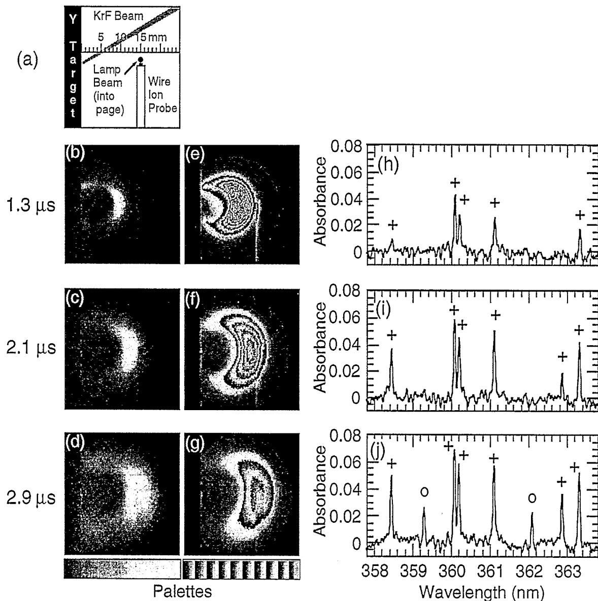
Fig. 3. Imaging and optical absorption spectra at the first peak, shoulder, and second peak of the ion probe waveform of Fig. 1(d) for yttrium ablation into 200 mTorr argon. (a) Schematic of the side-on view of the Y-target and focusing sheet of KrF-irradiation, wire ion probe at d = 1.5 cm, and position of Xe-lamp beam (propagating into the page) used for optical absorption spectroscopy just above the wire probe tip. (b)-(g) Gated ICCD photographs of the total visible optical plasma emission, 50 ns gates: (b)-(d) utilize the grayscale palette and are independently normalized to 10,000, 20,000, and 38,000 counts, respectively, while (e)-(g) utilize the 10-gray-scale palette and are all normalized to 38,000 counts. (h)-(j) Time-resolved optical absorption spectra ( \sim 2 cm optical path length, d = 1.5 cm, 100-spectra averaged with 200 ns gates centered at the imaged times) in 200 mTorr argon show that ground-state \text{Y}^+ ion lines (indicated by +) dominate absorption at (c) 1.3 \mu\text{s} and (b) 2.1 \mu\text{s} (first peak, shoulder of ion probe signal): 358.45, 360.07, 360.19, 361.10, 362.87, 363.31 nm. Y neutral absorption becomes (indic. by \circ ) noticeable in the second peak of the ion probe signal as indicated in (k) 2.9 \mu\text{s} , at 359.29, 362.09 nm.
