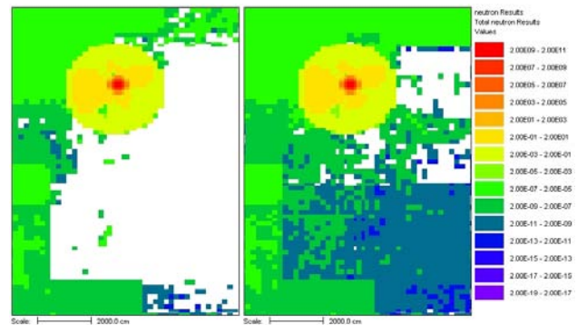
Fig. 2. Dose rates (mrem/h) computed using CADIS with the adjoint source on the outer boundaries of the model (left) and using FW-CADIS (right).
