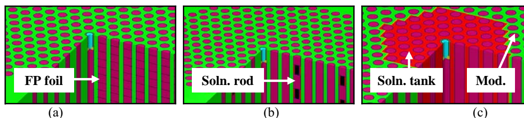
Fig. 1. Example assembly cutaways: (a) FP foils in between fuel pellets, (b) experimental rods with varying FP solution patterns, and (c) FP solution tank extending the length of the rods.
