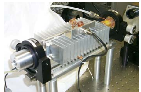
Waveguide CO 2 Laser Prototype.
