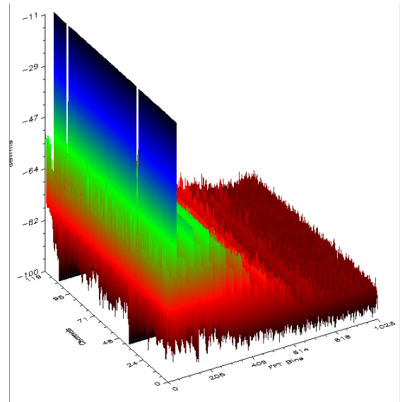
Graphical analysis of 120 channels of sensor data quickly allows identification of dead sensors.
